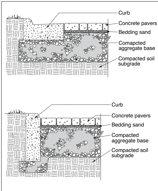
Figure 7. Poured in place concrete curbs.
