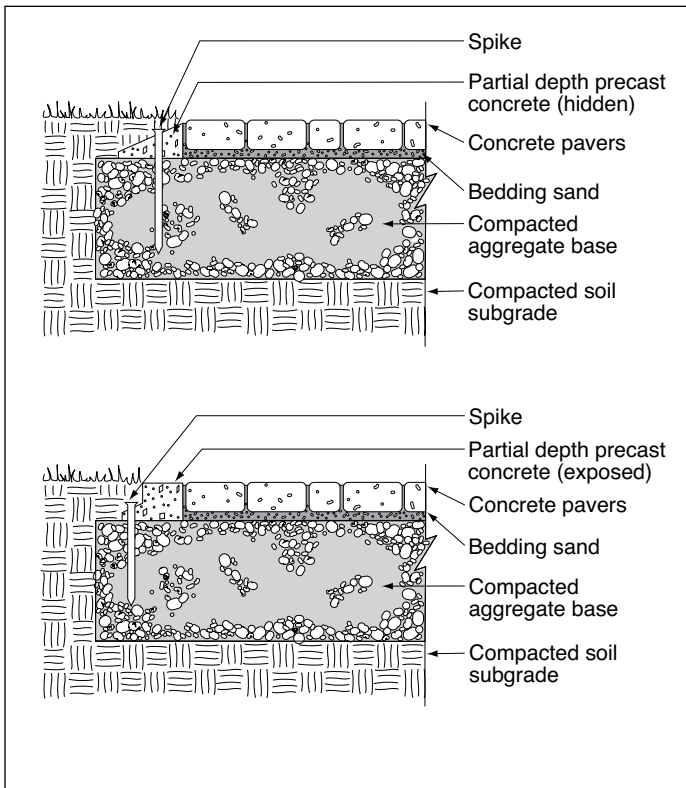
Figure 4. Partial depth precast concrete edge.
