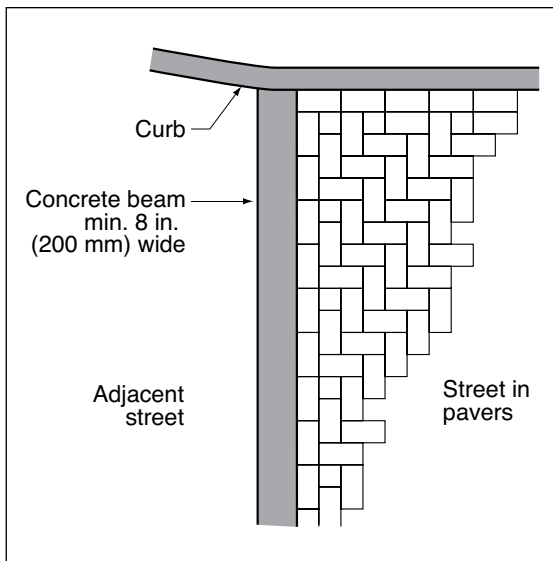
Figure 11. Concrete beam.
