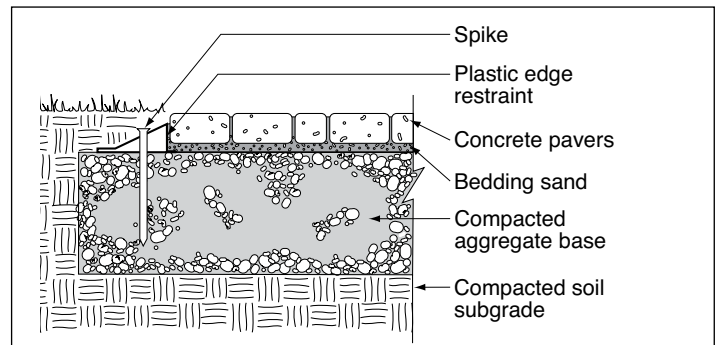
Figure 6. Plastic edge restraint.
