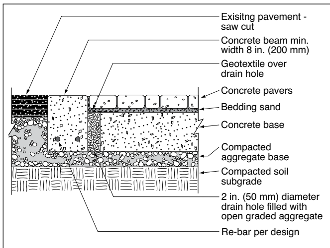
Figure 12. Crosswalk with concrete base.
