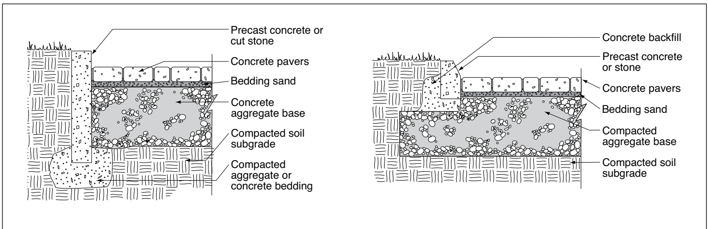
Figure 3. Precast concrete/cut stone.
