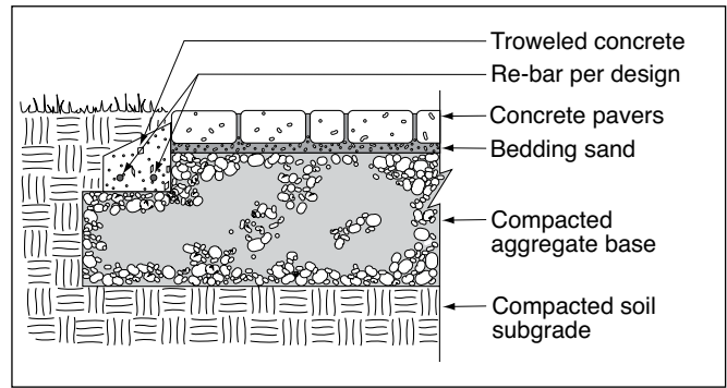
Figure 8. Troweled concrete edges.
