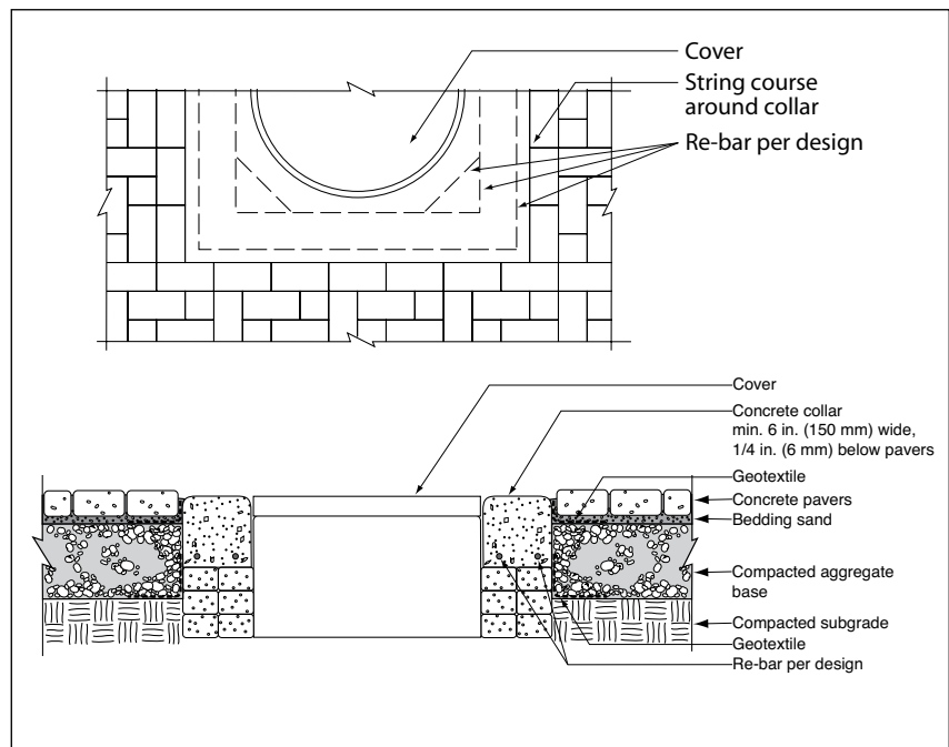
Figure 10. Utility cover.
