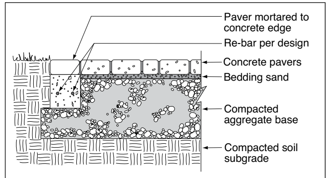
Figure 9. Submerged concrete edge.
