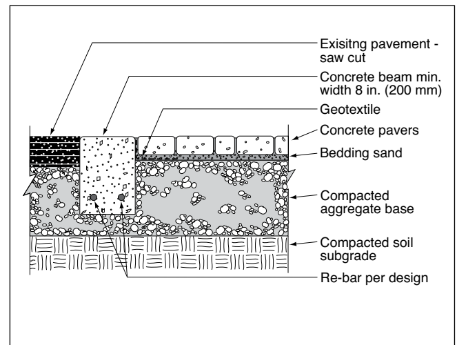
Figure 13. Crosswalk in existing asphalt pavement.
